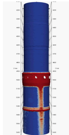
Wellhead Erosion
