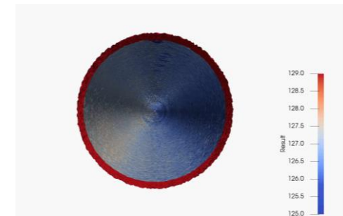
Casing Corrosion/Erosion
